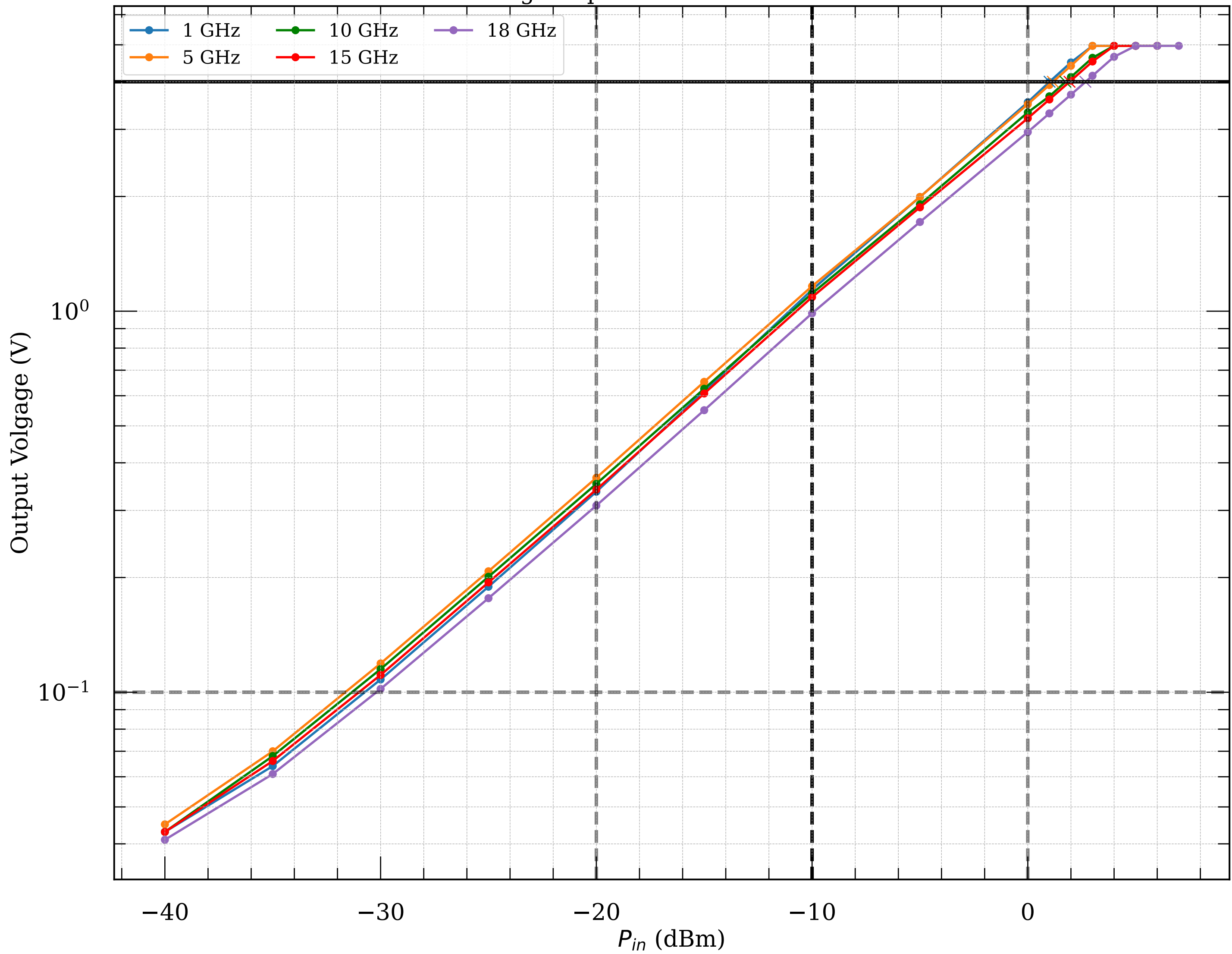
Measured voltage-to-power curve of detector module025
